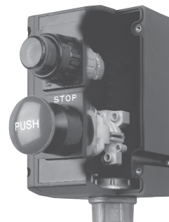
Maintained pushbutton with pilot light control station
