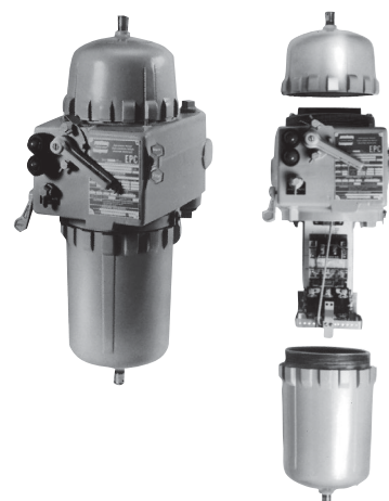
Assembled unit
