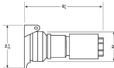
Connector
