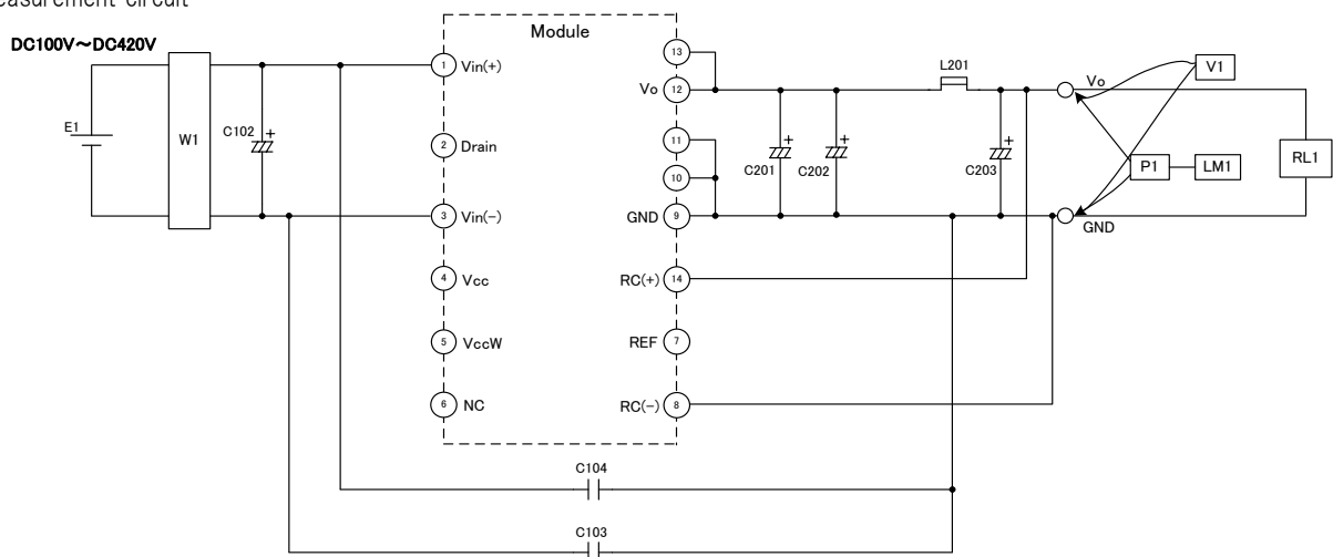
Measurement circuit
