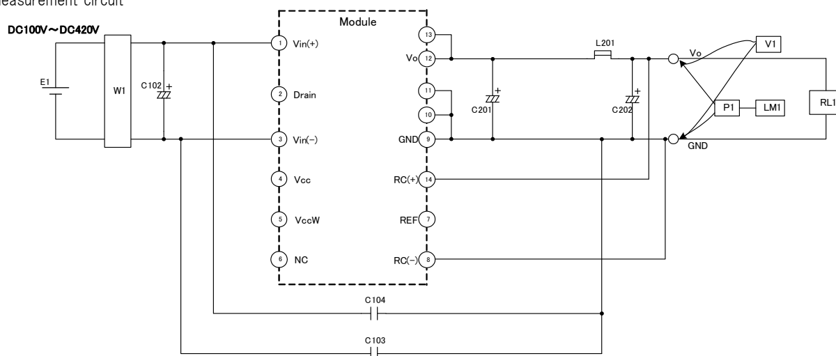
Measurement circuit
